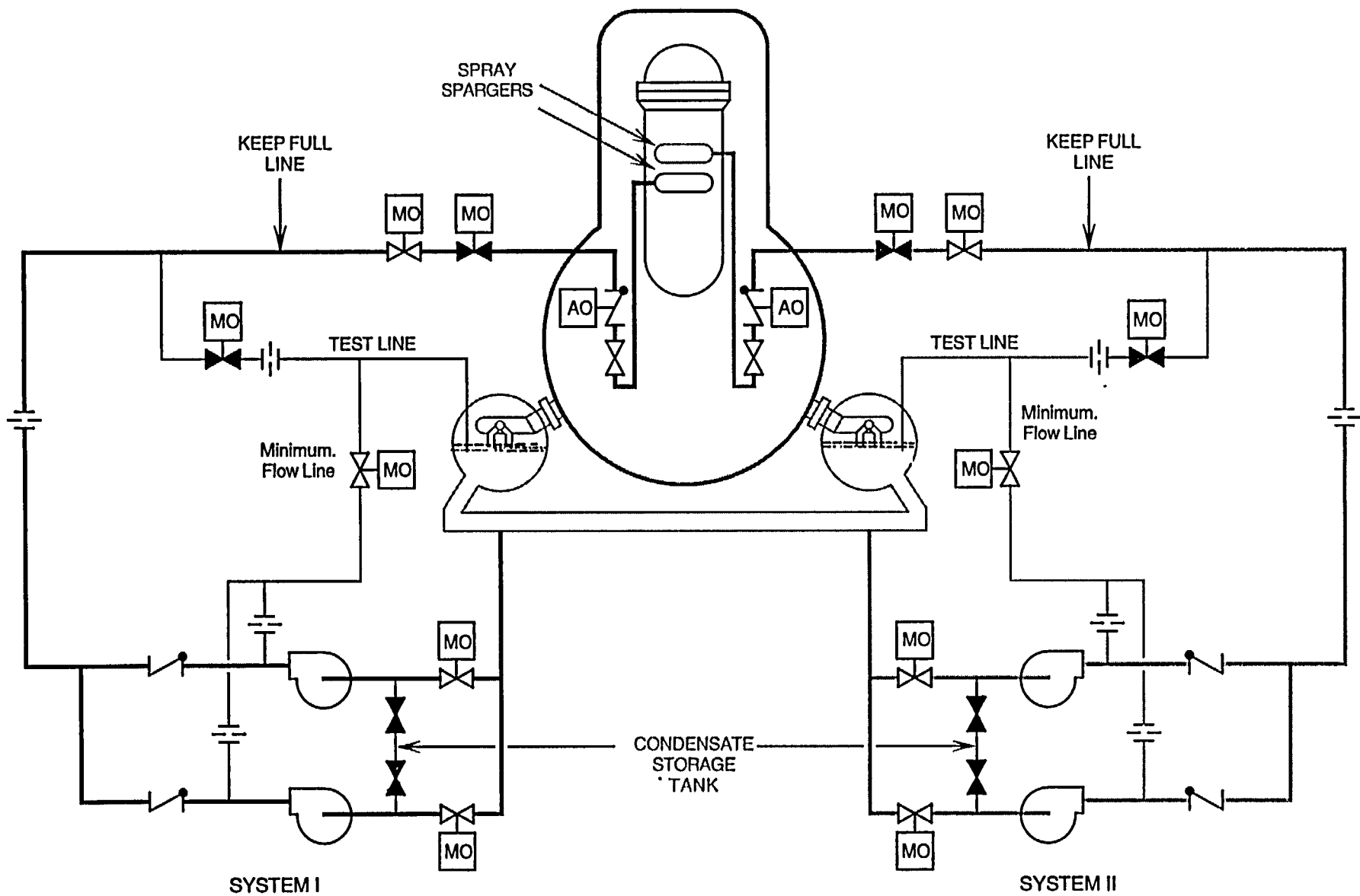
Figure 6.4-4 Core Spray System (BWR/3/4)
