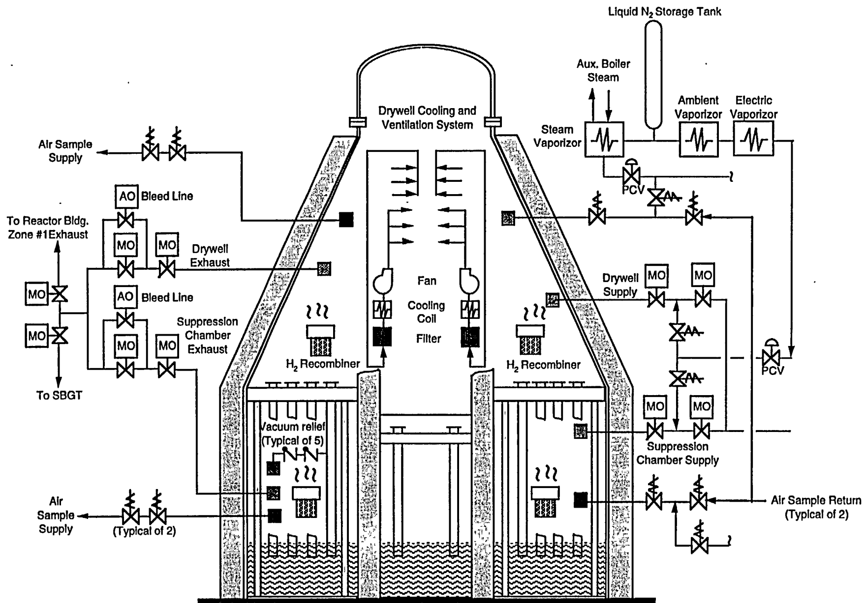
Figure 6.5-4 MARK II Containment Combustible Gas Control
