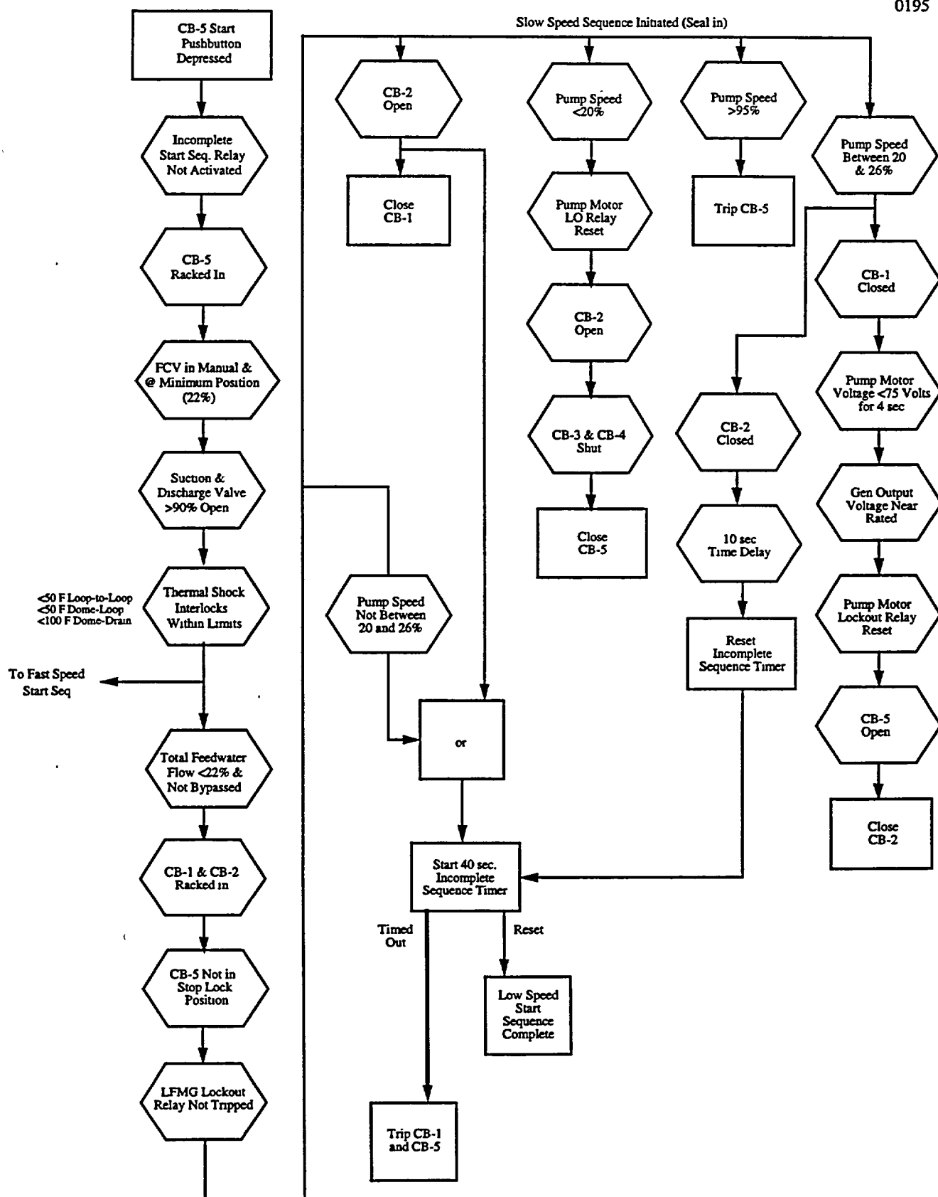
Figure 6.2-9 BWR/5 &amp; 6 Slow Speed Start Sequence
